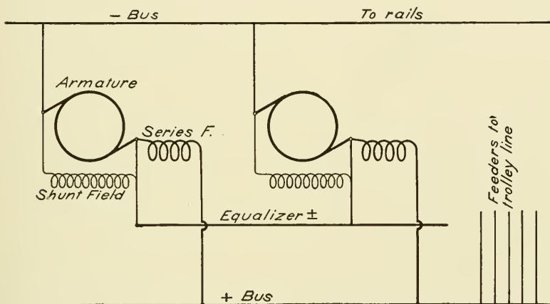
Fig. 150. Diagram of Connections for Direct-Current Power Plants
